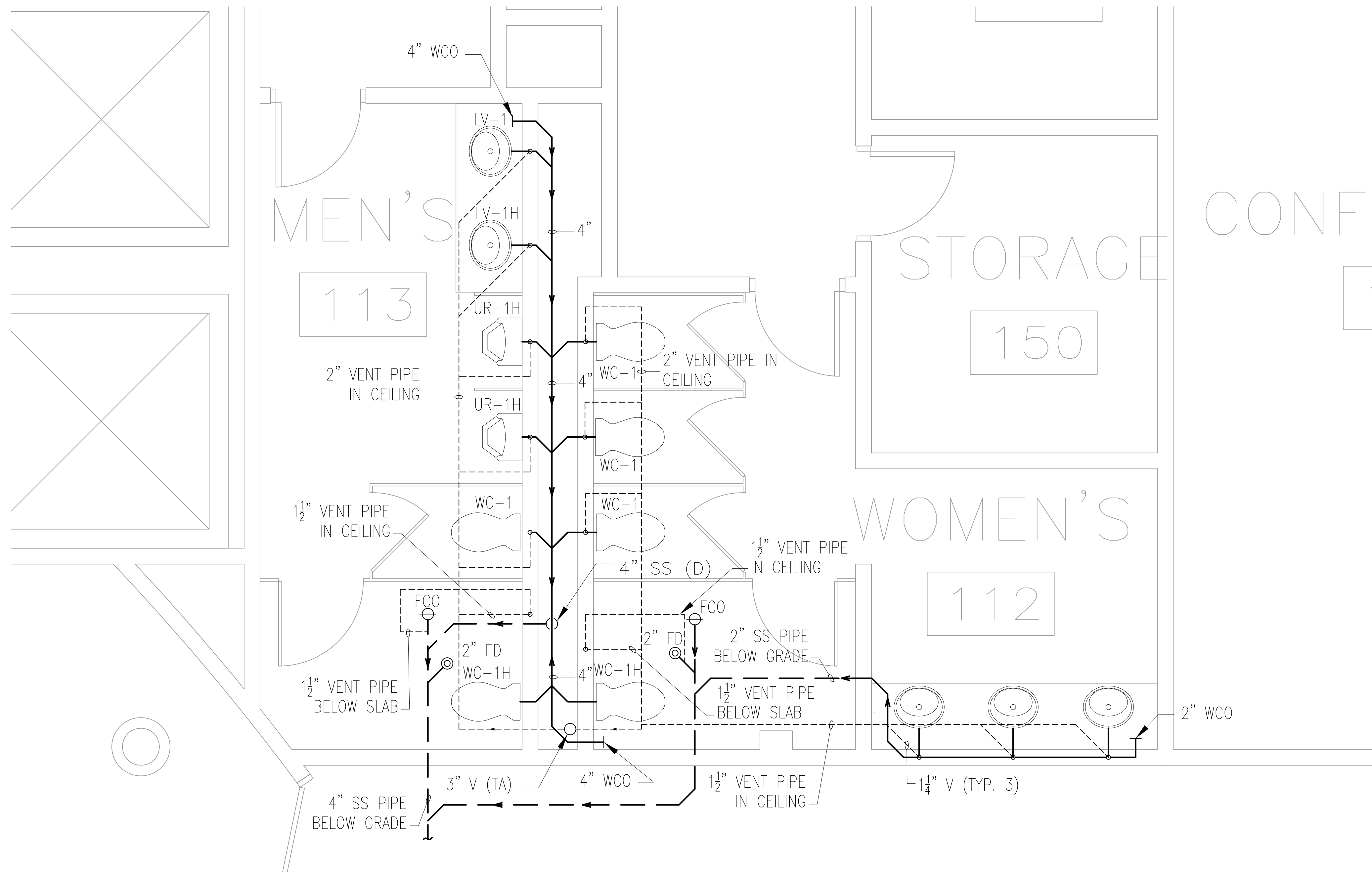
2 SANITARY — RESTROOM LAYOUT 1/2"=1'
