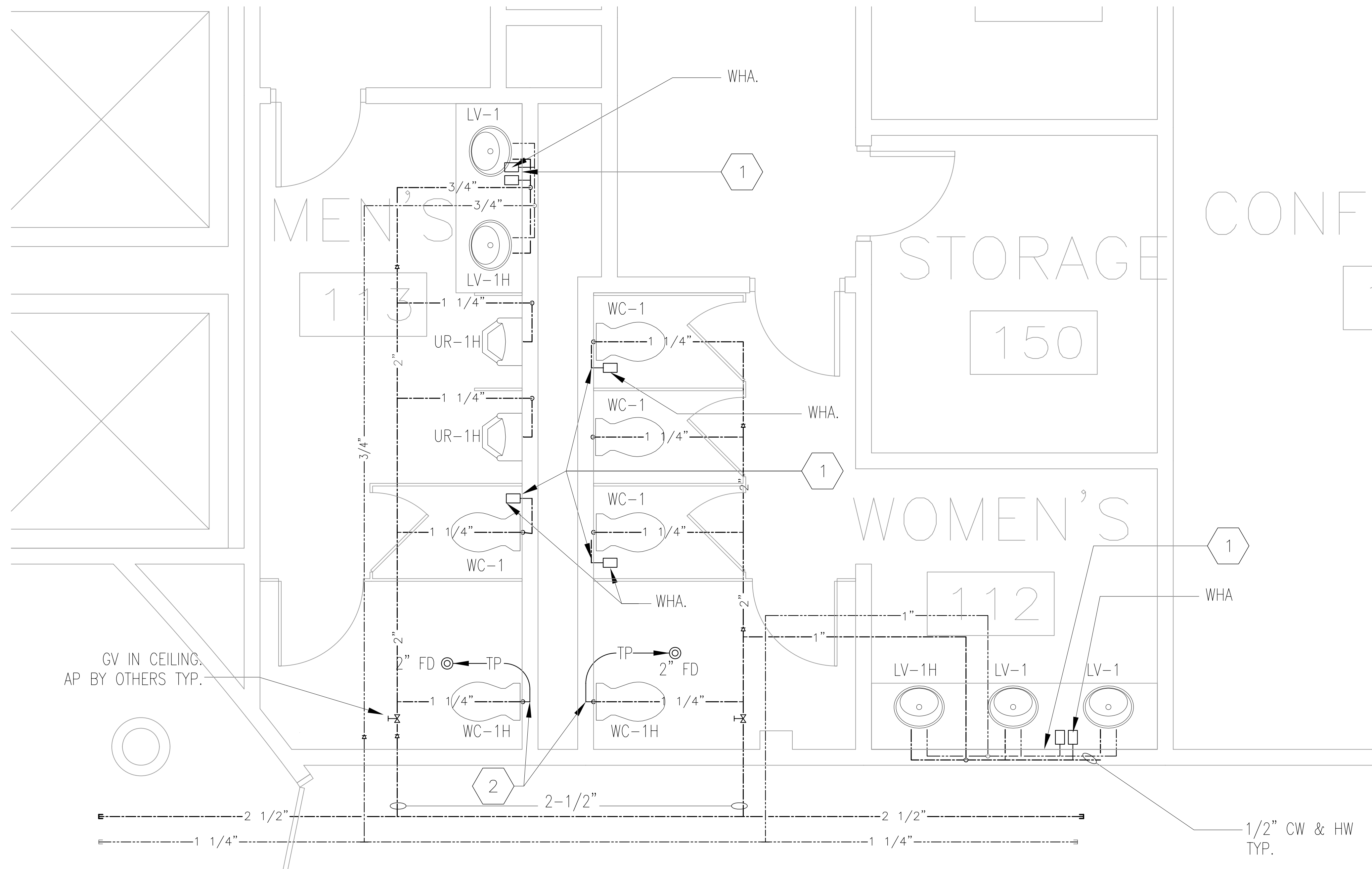
① COLD AND HOT WATER — RESTROOM LAYOUT 1/2"=1'
